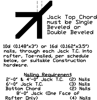
Connection Detail "C" (Top Chord to Hip Jack)
