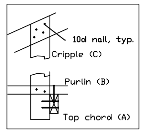
Cripple Connections
