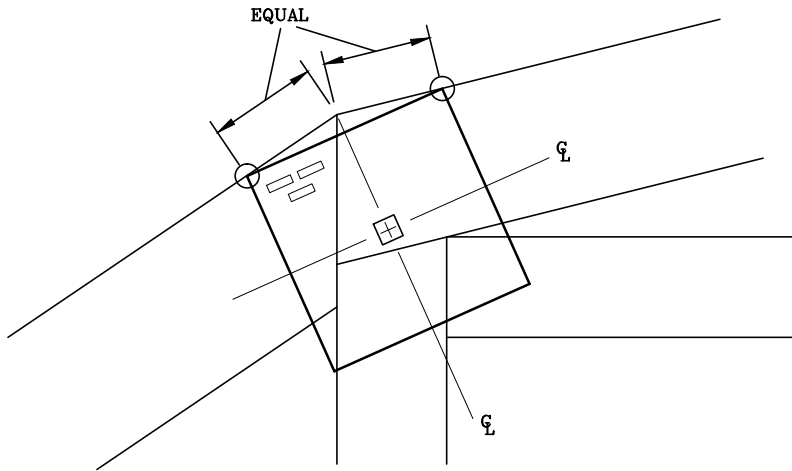
PLUMB/STANDARD JOINT
