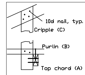
Cripple Connections
