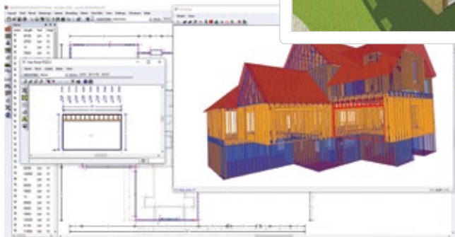
3D geometry is accurately transferred to the IntelliVIEW Suite to expedite the truss and panel framing process
