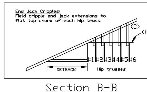
Cripple Connections
