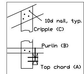
Cripple Connections
