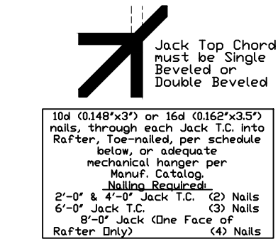
Connection Detail "C" (Top Chord to Rafter)
