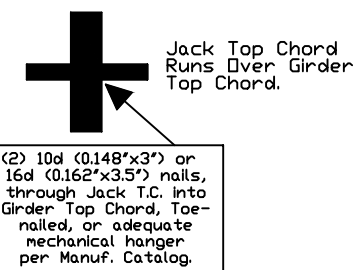
Connection Detail "A" (Top Chord to Hip Girder)
