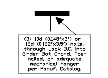
Connection Detail "B" (Bot Chord to Hip Girder)
